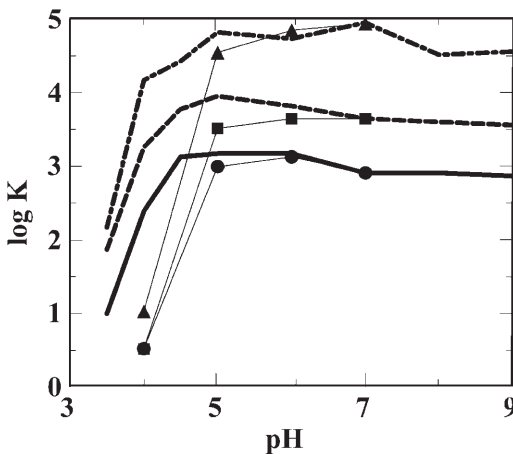
FIGURE 6 Influence of peptide charge on CaM binding at different pH values. Simulated curves representing the behavior of different peptides K4QK7QR17Q (solid line and filled circles), K7G (dashed line and filled squares) and smMLCK-am-ac (dot-dashed line and solid triangles). For each peptide, the log K shift ( \Delta \log K ) is calculated relative pH 7; C_s = 1.1 and C_p = 0.1 mM. Fat curves without symbols are obtained with a titratable protein, whereas curves with symbols are obtained with a fixed charge distribution on all amino acid residues. Note that the absolute value of log K has no meaning; only differences between the simulated numbers are of interest.
